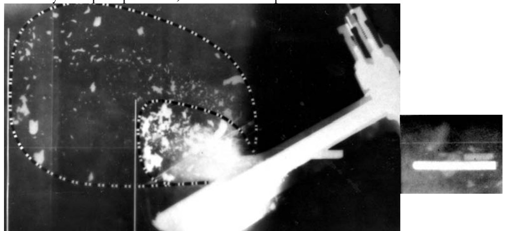
Image of steel rod penetrating steel plate, obtained by flash radiography.
